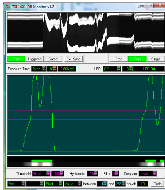
Figure 3: TSL1401_Monitor GUI
